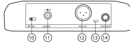
Rear Panel
